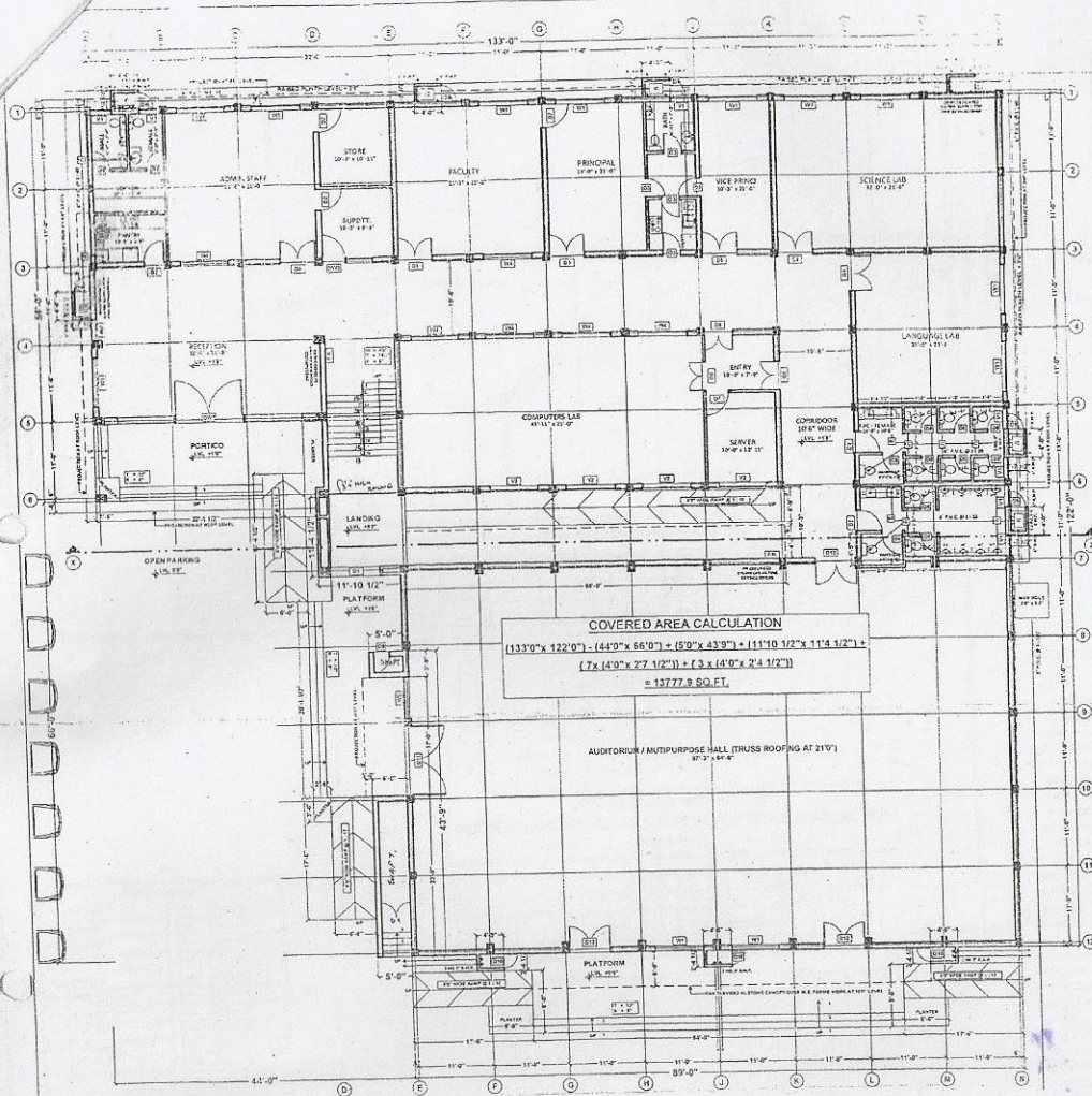
GROUND FLOOR PLAN SCALE 1" = 8'0"
