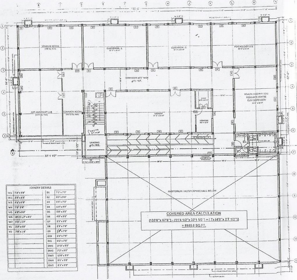
FIRST FLOOR PLAN SCALE 1" = 8'0"
